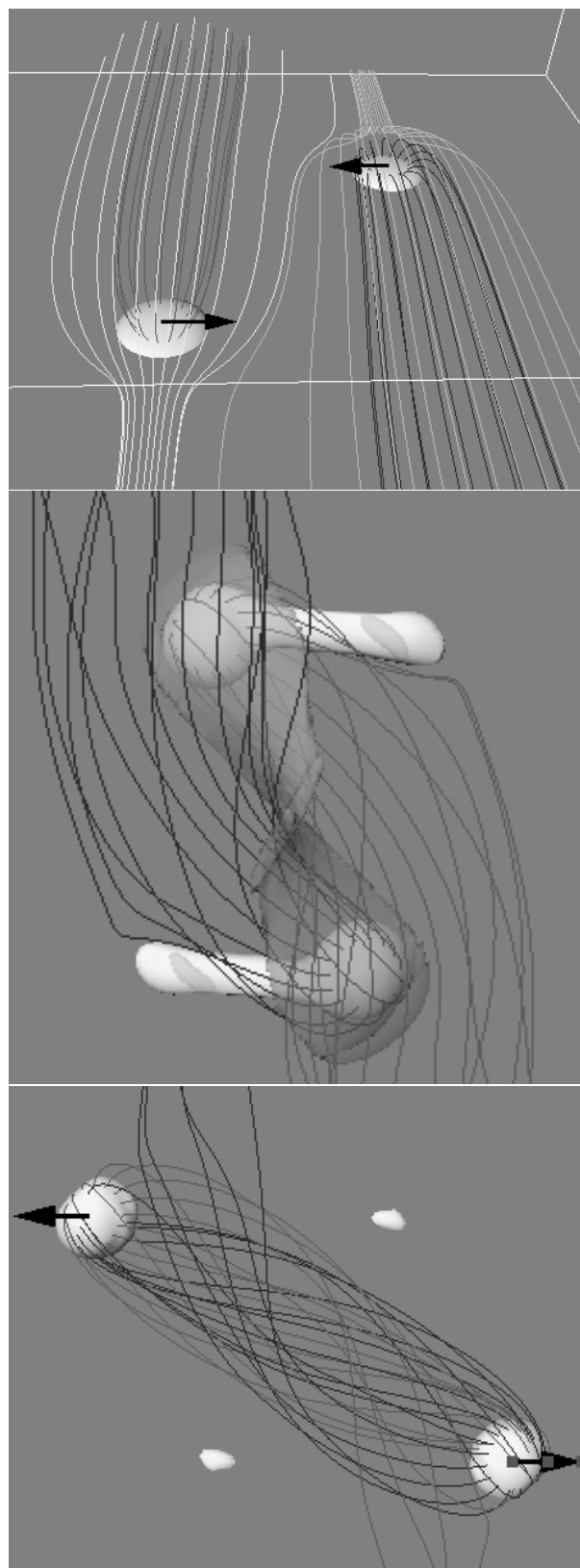
Fig. 7. Numerical experiment on separator reconnection, showing (a) the initial state, (b) the current sheet during reconnection and (c) the final state (Galsgaard et al. , 2000).
